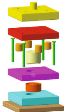
3-D Tool Modeling of Stamping Part Spring Sheet
